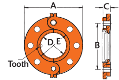
2" - 12" (hinged)
