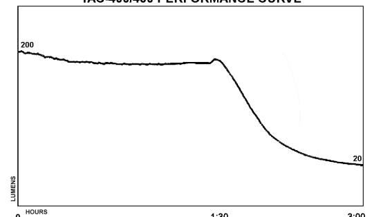
TAC-400/450 PERFORMANCE CURVE
