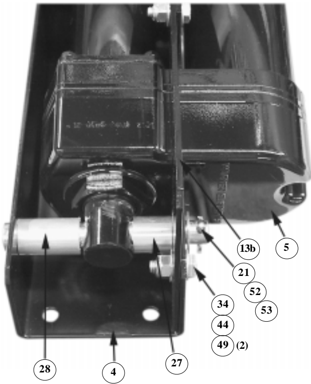
FIGURE 4 - ACTUATOR
