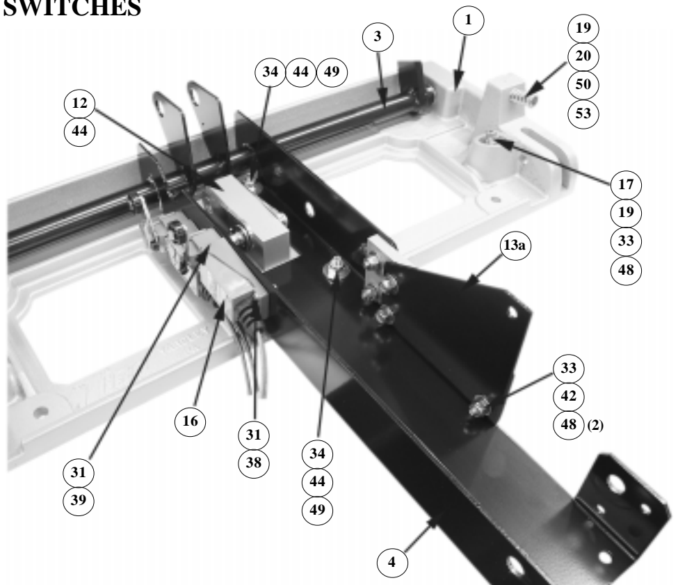
FIGURE 7 - MICRO SWITCHES
