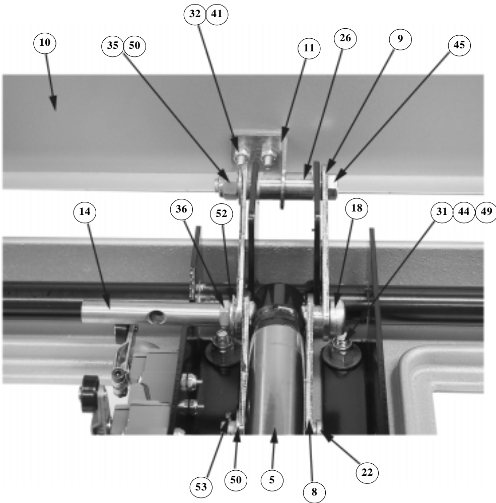
FIGURE 8 - LOWER ASSEMBLY
