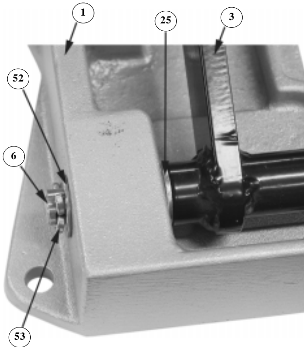
FIGURE 5 - TORQUE TUBE
