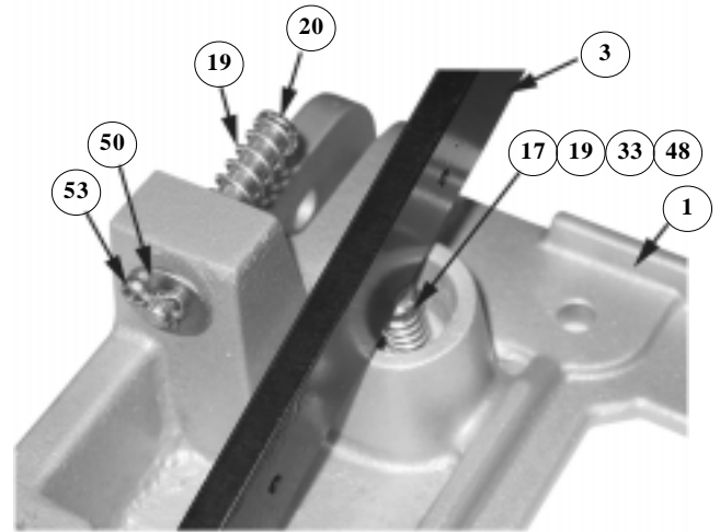
FIGURE 12 - SPRINGS
