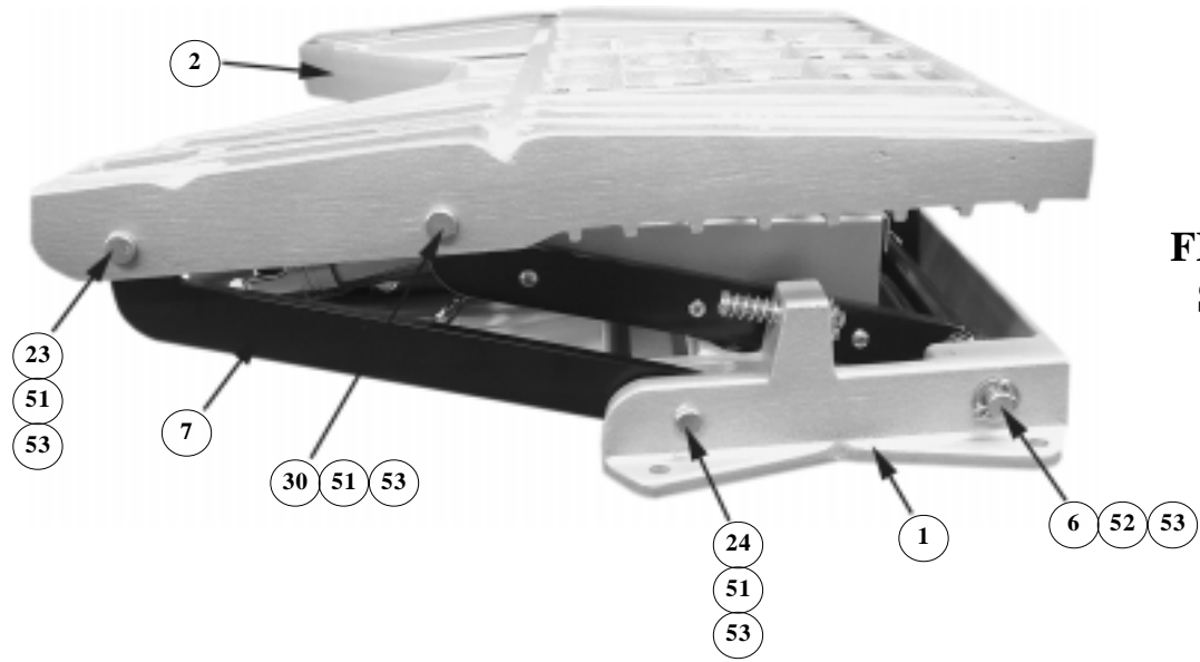
FIGURE 11 - STEP
