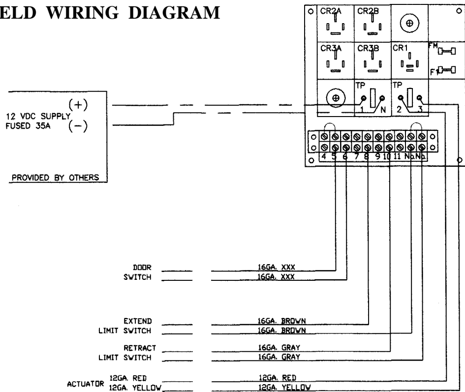
FIGURE 2 - ELECTRICAL SCHEMATIC
