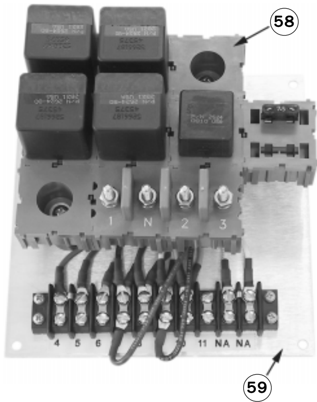
FIGURE 3 - ELECTRICAL PANEL
