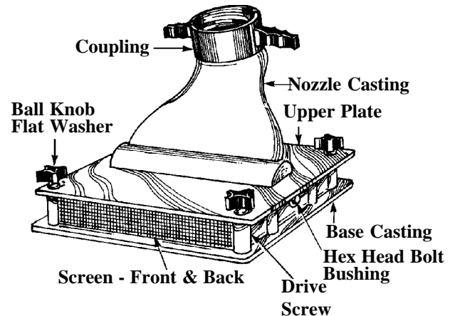
Model QD-250
