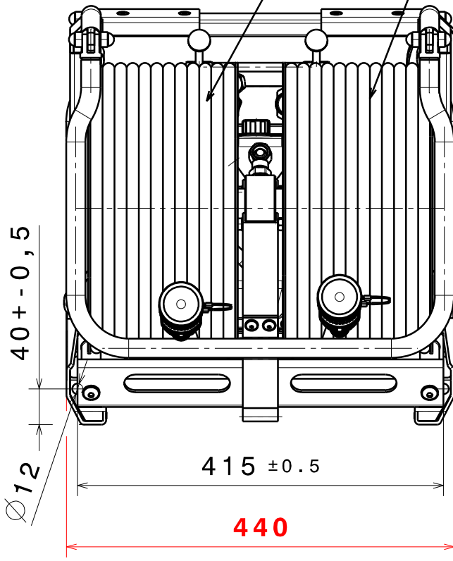
Schlauchpaar 20m rot PAIR OF HOSES RED 20m
