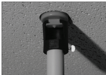
Figure 1: Attach Sprinkler Wrench 14031 onto a length of 1" diameter CPVC pipe
