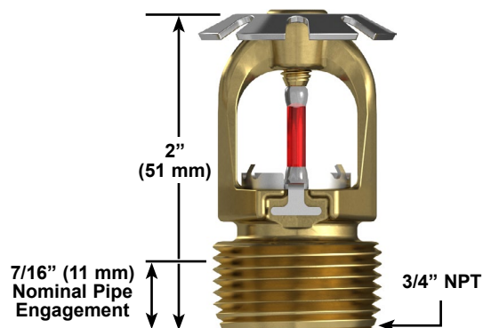
Figure 2: Sprinkler Dimensions
