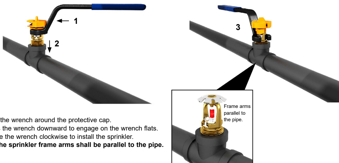
Figure 3: Installation
