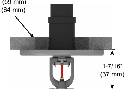
Standard Surface-Mounted Escutcheon
