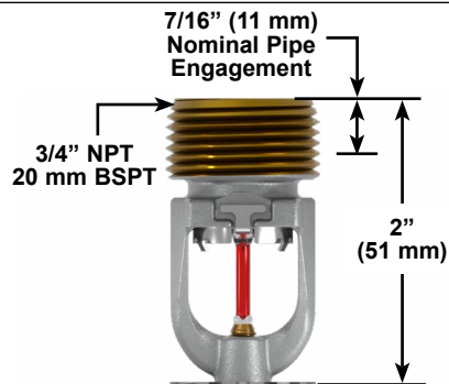
Figure 2: Sprinkler Dimensions
