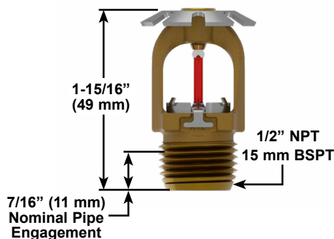
Figure 2: Sprinkler Dimensions
