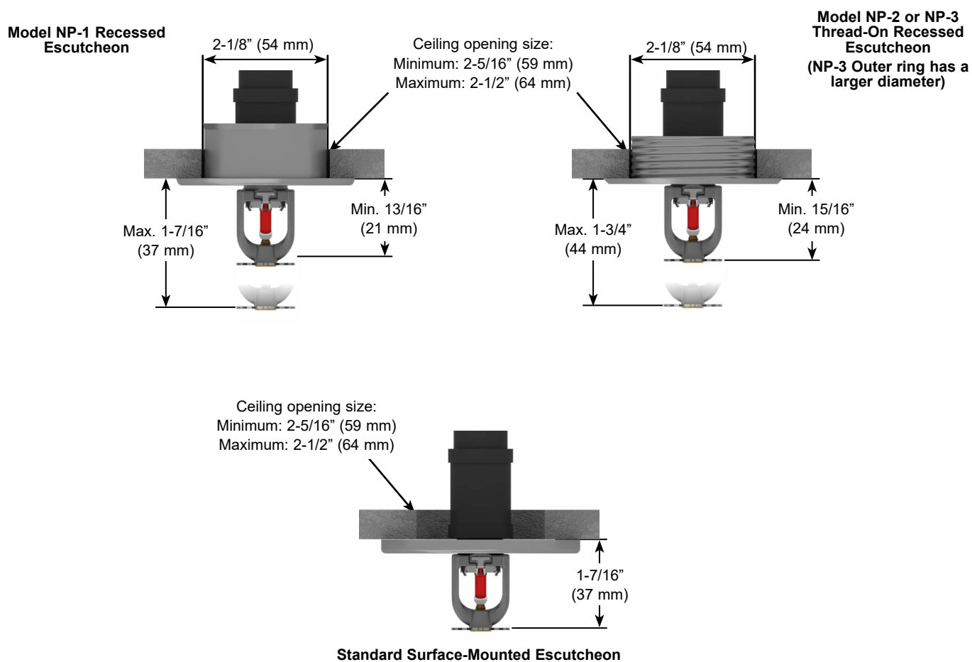
Figure 5: Installation Dimensions with Viking Escutcheons
