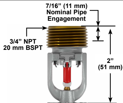
Figure 2: Sprinkler Dimensions
