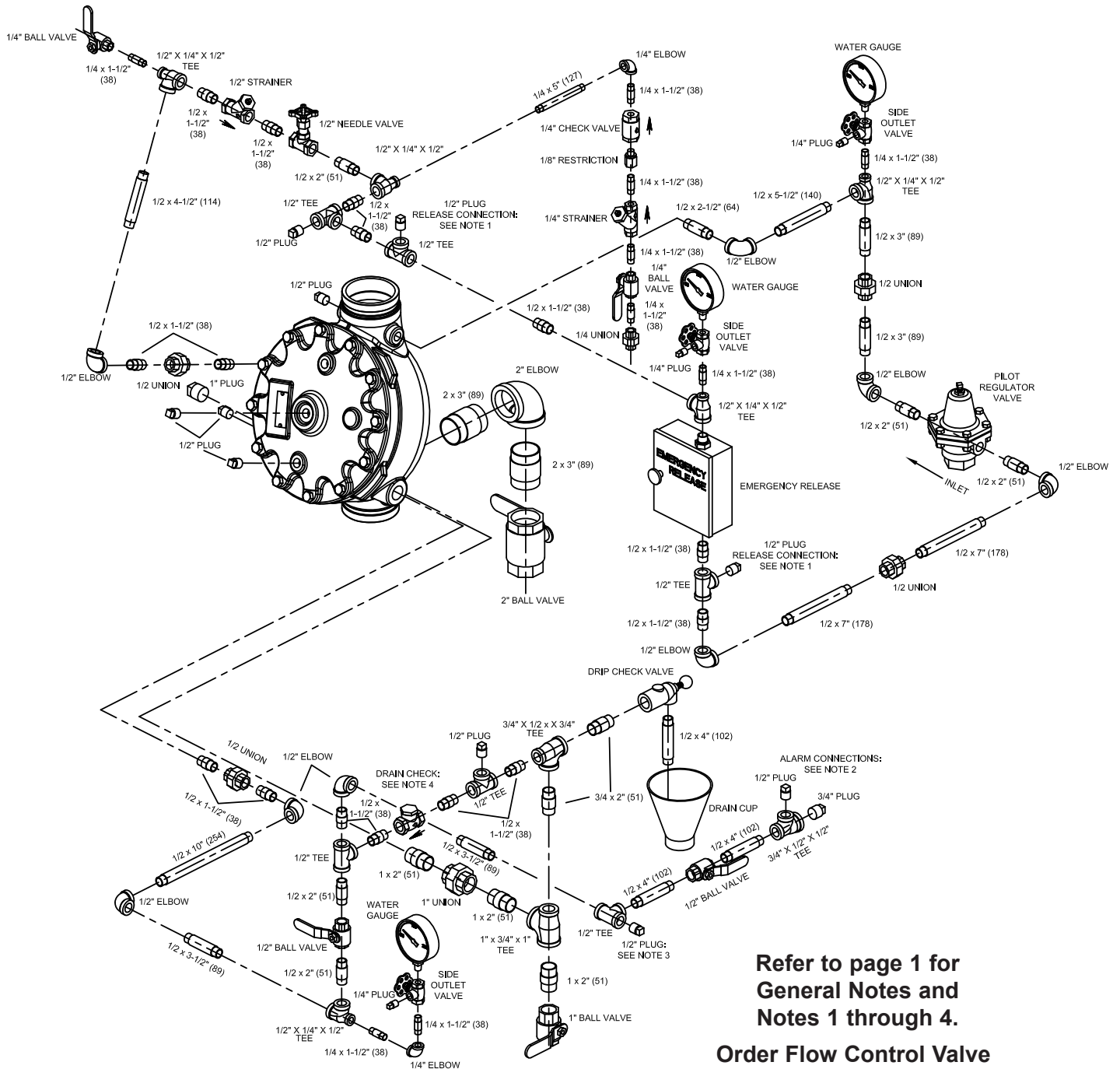
Figure 1 4" Pilot Regulating Trim for Model J Flow Control Valve
