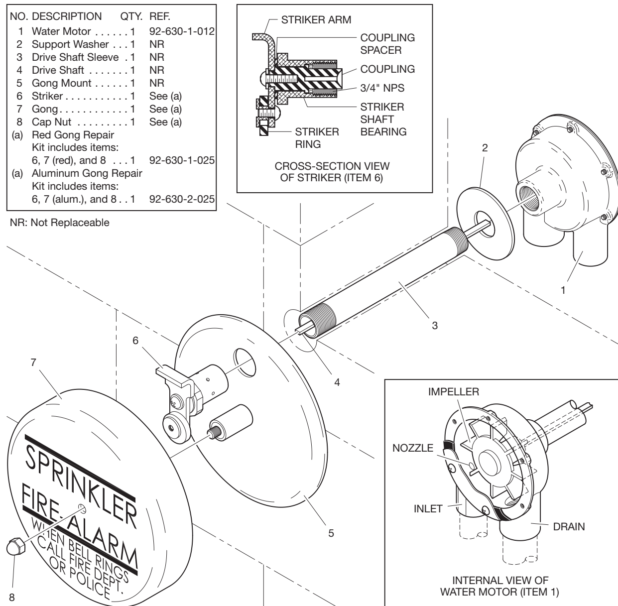
FIGURE 1 MODEL WMA-1 WATER MOTOR ALARM ASSEMBLY
