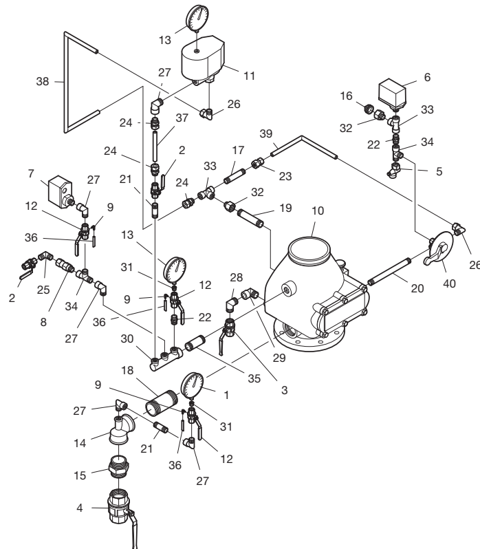
FIGURE 13 EUROPEAN CONFORMITY MODEL DPV-1 DRY PIPE VALVE TRIM with THREE-WAY ALARM TEST VALVE with MODEL ACC-1 ACCELERATOR — DN150 —
