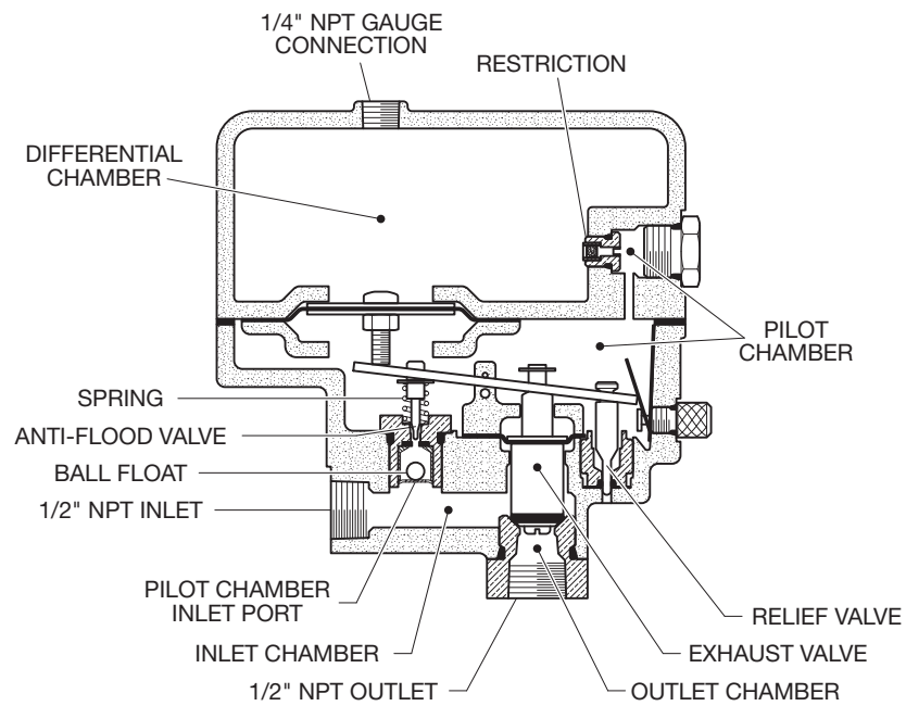
FIGURE 6 MODEL ACC-1 DRY PIPE VALVE ACCELERATOR — IN SET POSITION —
