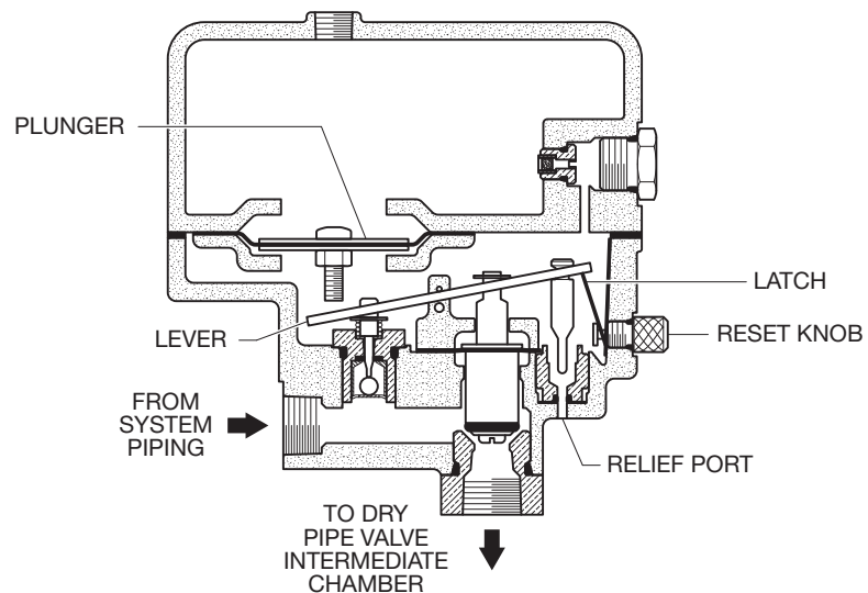
FIGURE 7 MODEL ACC-1 DRY PIPE VALVE ACCELERATOR — IN TRIPPED POSITION —
