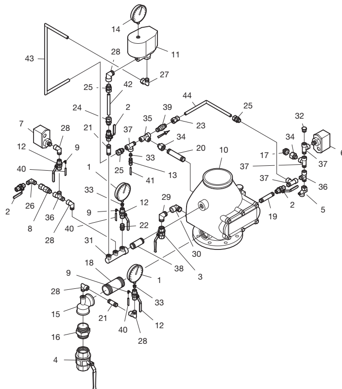
FIGURE 15 EUROPEAN CONFORMITY MODEL DPV-1 DRY PIPE VALVE TRIM with STANDARD ALARM TEST VALVE with MODEL ACC-1 ACCELERATOR — DN150 —
