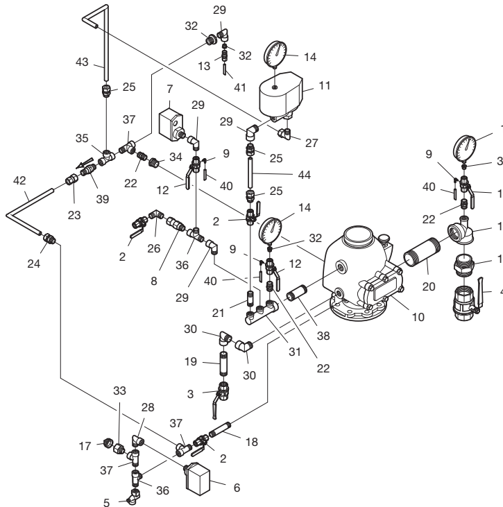
FIGURE 14 EUROPEAN CONFORMITY MODEL DPV-1 DRY PIPE VALVE TRIM with STANDARD ALARM TEST VALVE with MODEL ACC-1 ACCELERATOR — DN100 —
