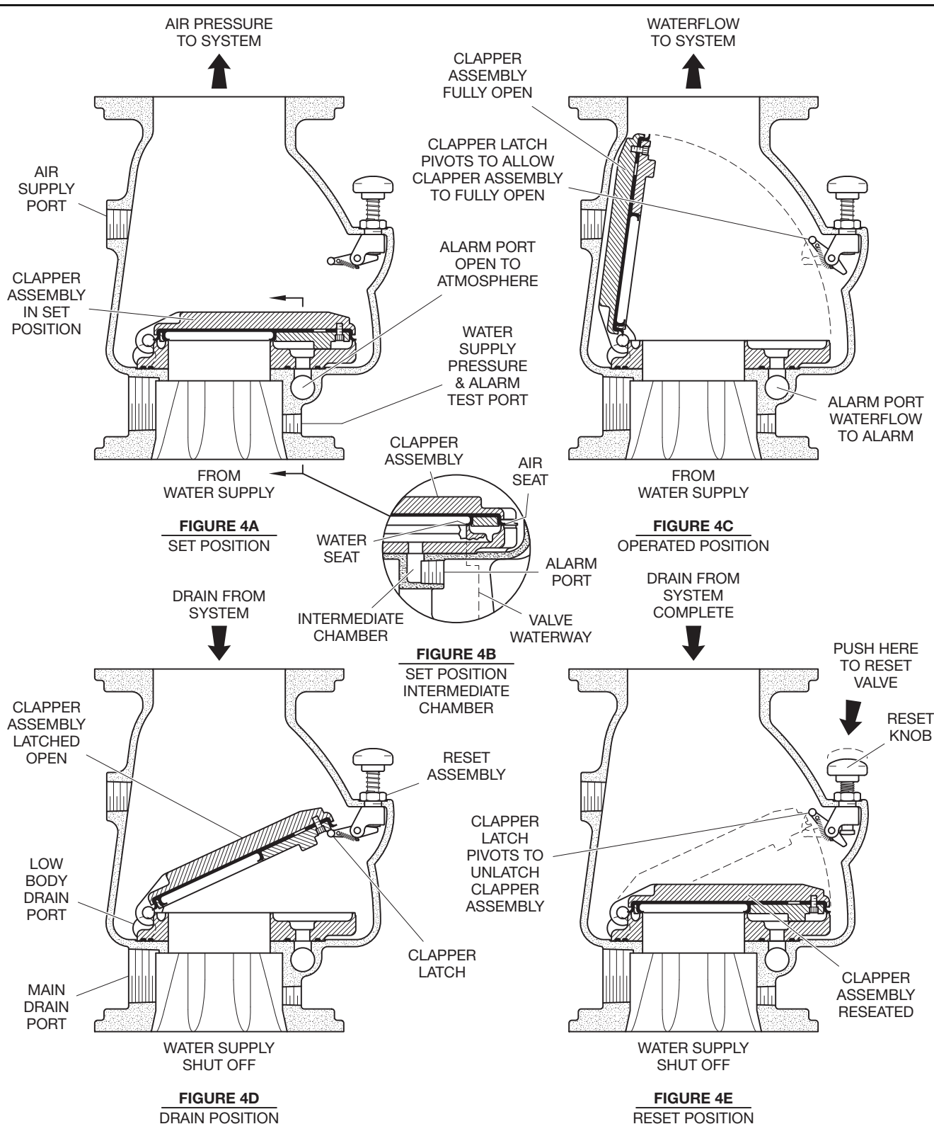
FIGURE 4 (2 of 2) DN150 MODEL DPV-1 DRY PIPE VALVE — SET AND OPEN POSITIONS —
