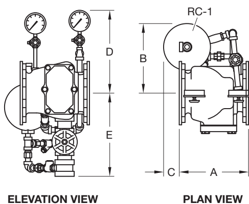
FIGURE 7 (2 OF 3) INSTALLATION DIMENSIONS FOR 4 & 6 INCH (DN100 & DN150) MODEL AV-1-300 ALARM CHECK VALVES
