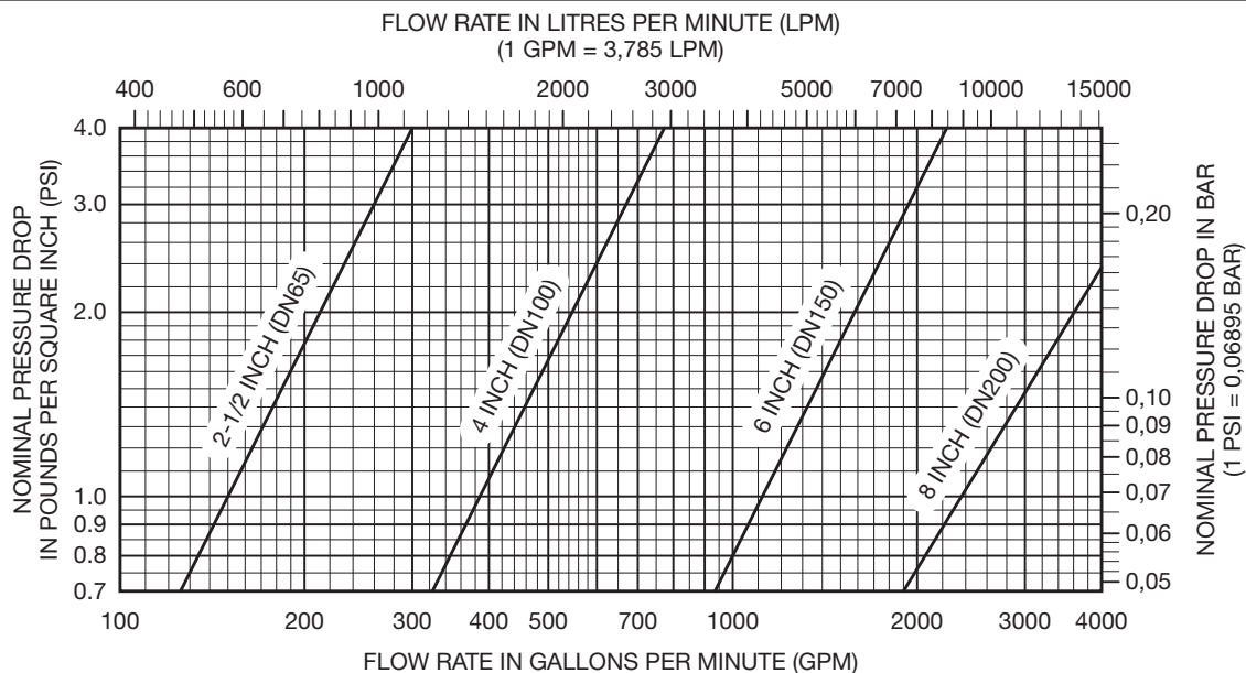
GRAPH A 2-1/2, 4, 6 & 8 INCH (DN65, DN100, DN150 & DN200) MODEL AV-1-300 ALARM CHECK VALVE NOMINAL PRESSURE LOSS VERSUS FLOW
