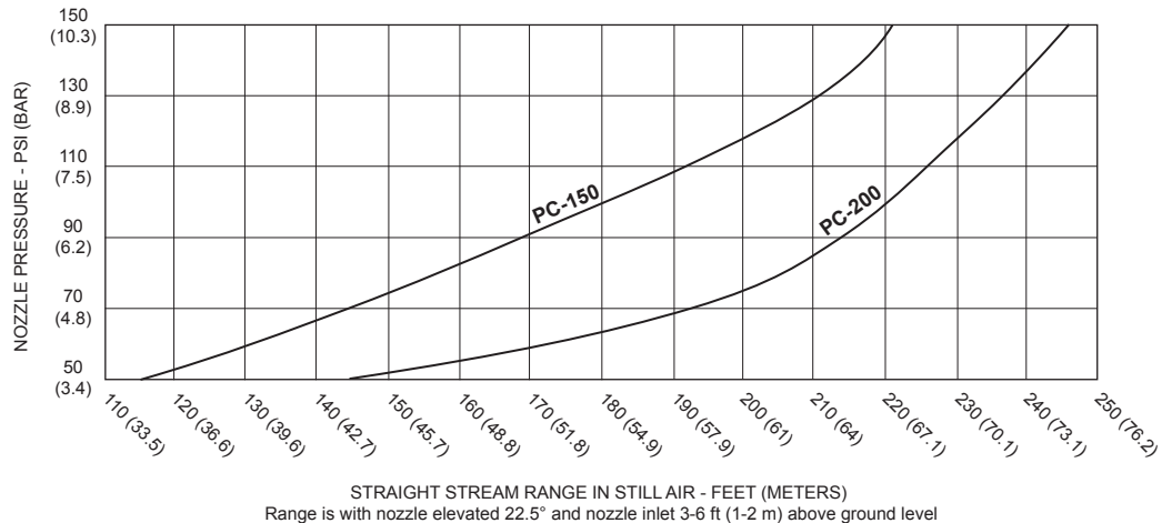
RANGE CHARACTERISTICS OF STRAIGHT STREAM NOZZLES
