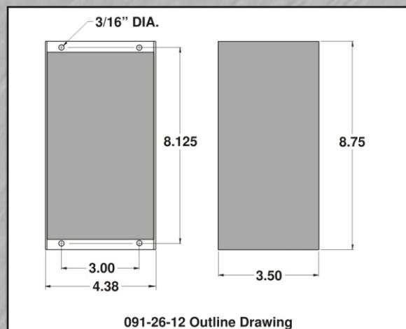
091-26-12 Outline Drawing
