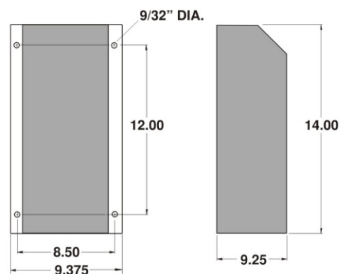
091-162-12 Outline Drawing
