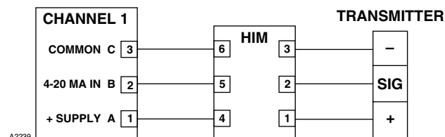
Figure 6—Three-Wire Transmitter / Detector with HART Interface Module — Non-Isolated 4 to 20 mA Current Output (Sourcing)
