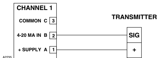
Figure 3—Two-Wire Transmitter / Detector — Non-Isolated 4 to 20 mA Current Output (Sourcing)
