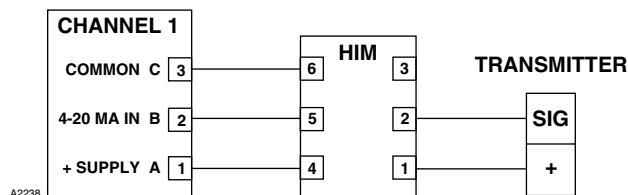
Figure 4—Two-Wire Transmitter / Detector with HART Interface Module — Non-Isolated 4 to 20 mA Current Output (Sourcing)
