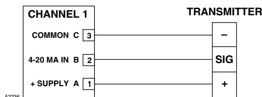
Figure 5—Three-Wire Transmitter / Detector — Non-Isolated 4 to 20 mA Current Output (Sourcing)
